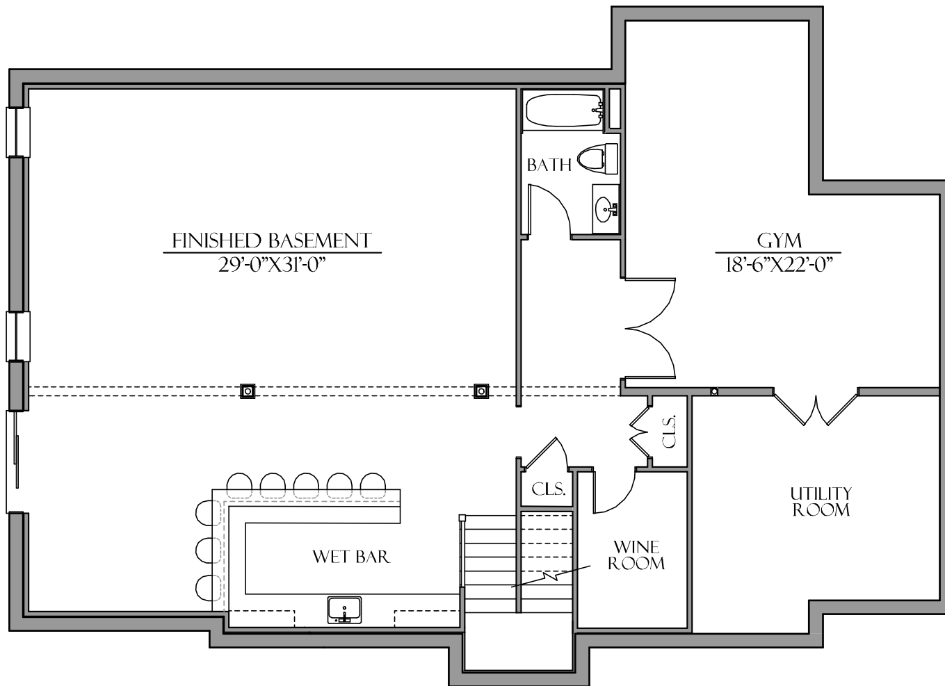
BASEMENT PLAN: TOTAL AREA = 1,590 S.F.
