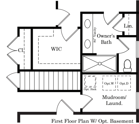
First Floor Plan W/ Opt. Basement
